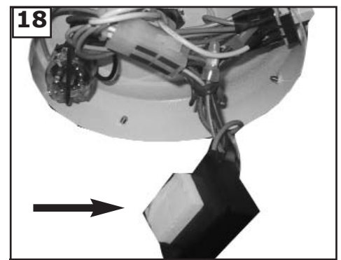
Black capacitor box needs to be stuck to the switch housing. Not being attached can cause motor noise.
