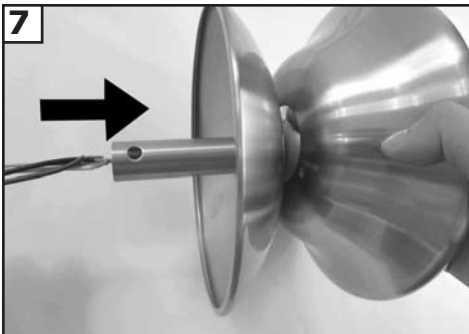
7 Thread leadwires and safety cable through the downrod.
