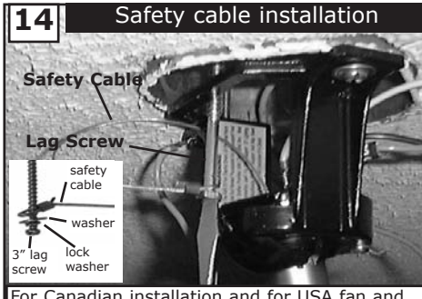
14 Safety cable installation For Canadian installation and for USA fan and light kit combinations over 35 lbs, in both flush and downrod mode the safety cable must be installed into the house structure beams using the 3" lag screws, washers, and lock washers provided. Make sure that when the safety cable is fully extended the leadwires are longer than the cable and no stress is placed on the leadwires.
