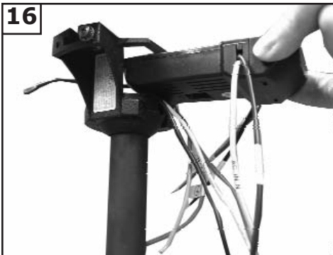
16 Install remote receiver into the mounting bracket.
